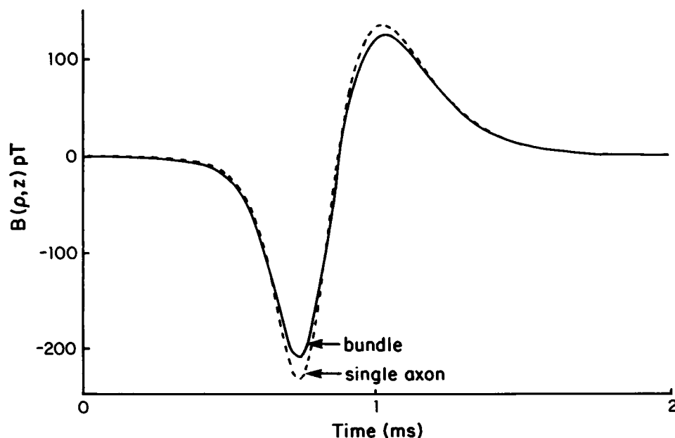
FIGURE 10 The magnetic field of an axon off-axis in a sheathed, anisotropic nerve bundle. a = 0.107 mm, \sigma_i = 1.70 \Omega^{-1} \text{ m}^{-1} , \sigma_s = 2.06 \Omega^{-1} \text{ m}^{-1} , \rho = 1.48 mm, u = 16.5 \text{ m/s}^{-1} , \sigma_r = 0.2 \Omega^{-1} \text{ m}^{-1} , \sigma_b^{\rho} = 2.0 \Omega^{-1} \text{ m}^{-1} , \sigma_b^z = 0.2 \Omega^{-1} \text{ m}^{-1} , b = 0.625 mm, c = 0.635 mm, t = 0.45 mm.
