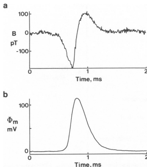
FIGURE 3 (a) The measured magnetic field, (b) the measured transmembrane potential. In both cases no signal averaging was used.
