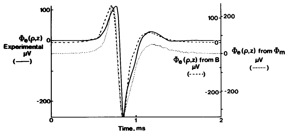
FIGURE 11 The external potential calculated from the transmembrane potential (dotted), calculated from the magnetic field (dashed), and measured (solid).
