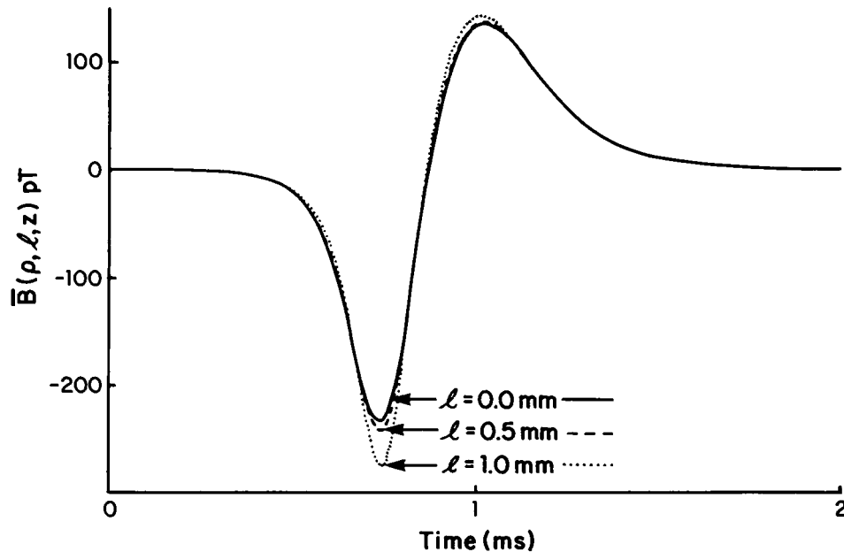
FIGURE 6 The magnetic field corrected for the axon being off-axis in the toroid. The distance off-axis, \ell , is equal to 0.0, 0.5, and 1.0 mm for the three traces. a = 0.107 mm, \sigma_i = 1.70 \Omega^{-1} \text{ m}^{-1} , \sigma_e = 2.06 \Omega^{-1} \text{ m}^{-1} , \rho = 1.48 mm, u = 16.5 m/s.
