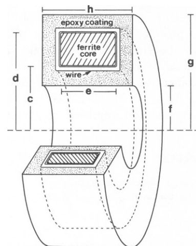
FIGURE 2 Geometry of the toroid; c = 1.05 mm, d = 1.95 mm, e = 1.25 mm, f = 0.75 mm, g = 2.25 mm, and h = 1.90 mm.
