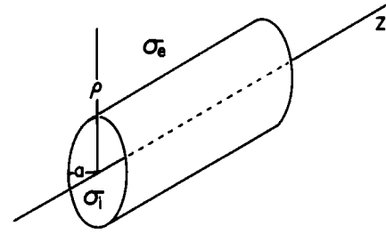
FIGURE 14 The geometry of a nerve axon.
